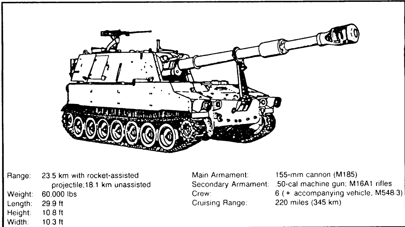
Figure 7-40. M109A2/A3 SP howitzer
