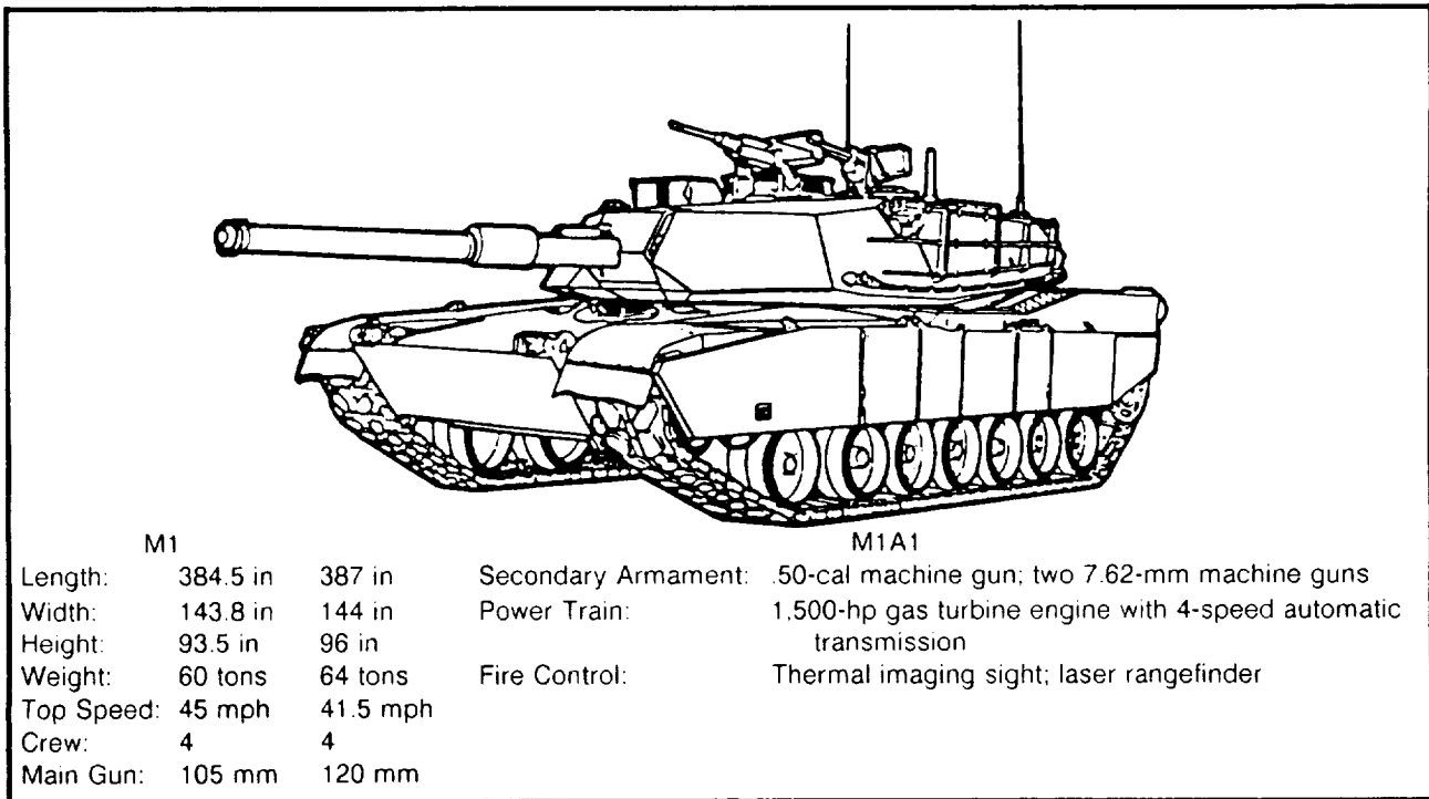
Figure 7-34. M1 Abrams tank
