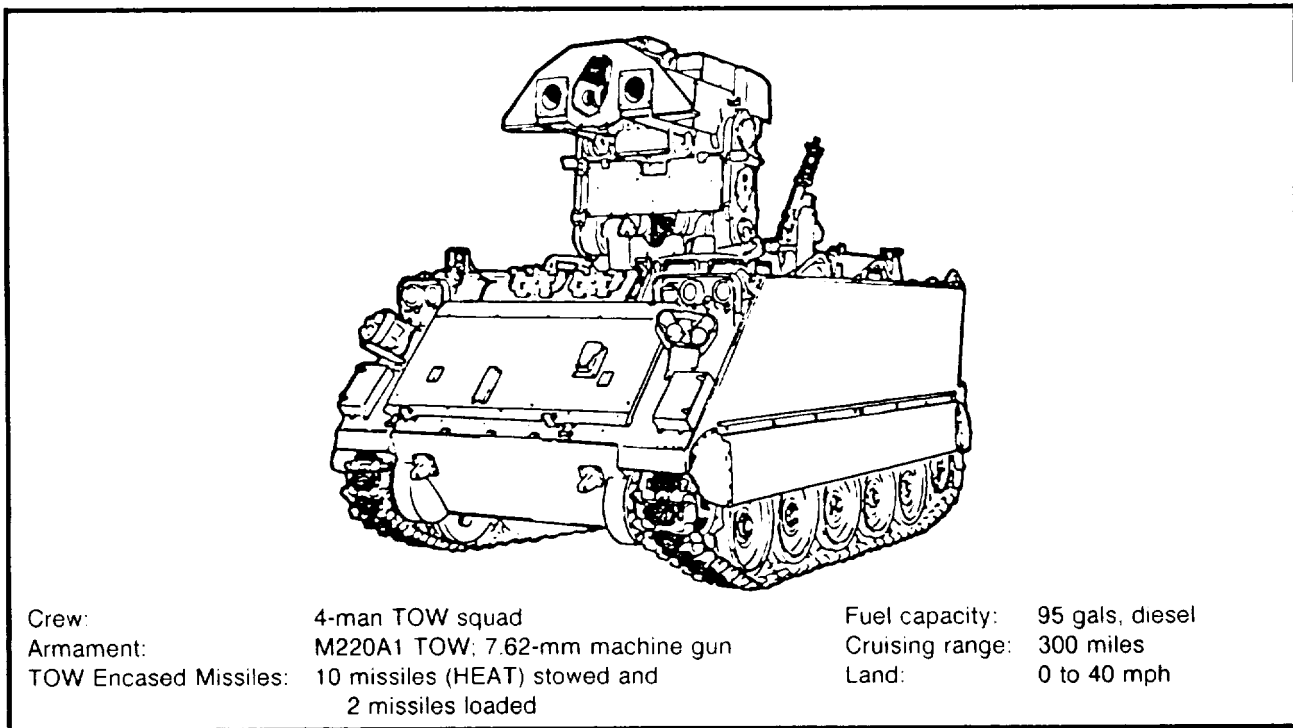
Figure 7-38. M901 improved TOW vehicle
