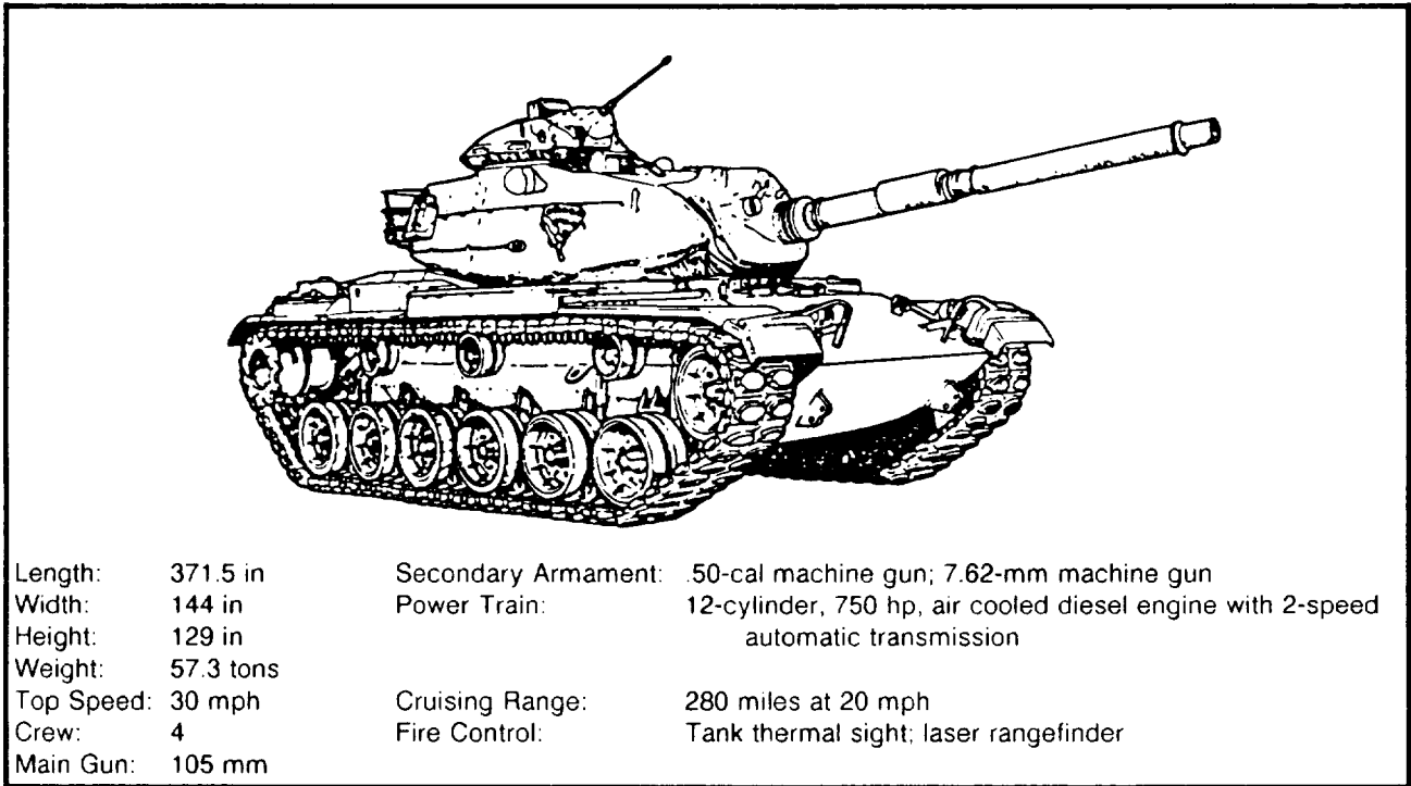
Figure 7-35. M50A3 tank
