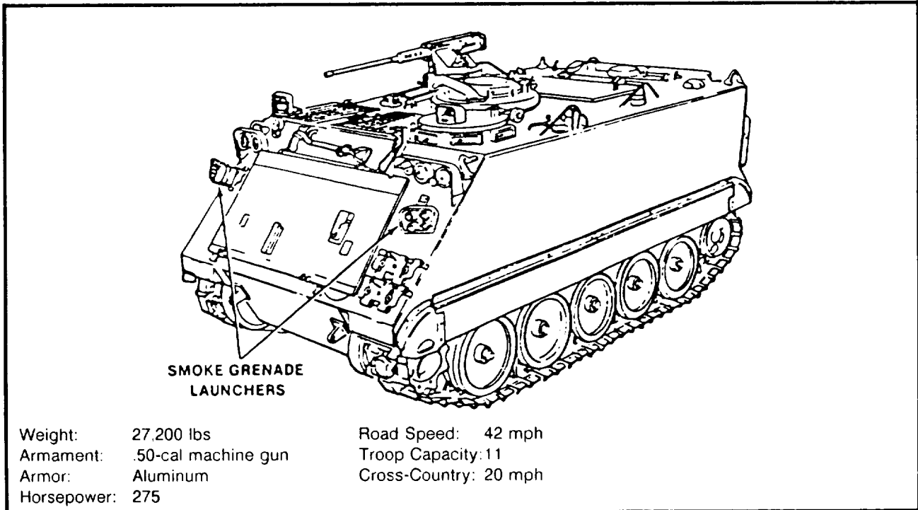
Figure 7-37. M113 armored personnel carrier
