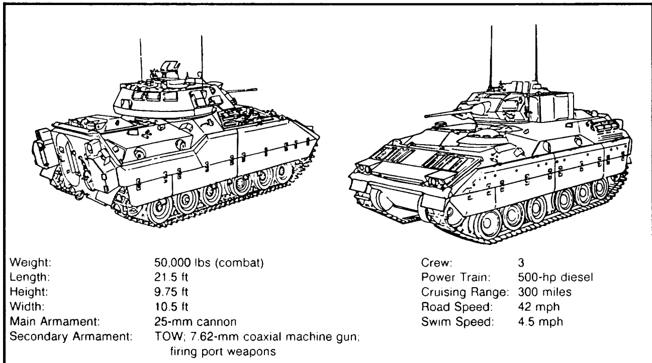
Figure 7-36. M213 Bradley fighting vehicle
